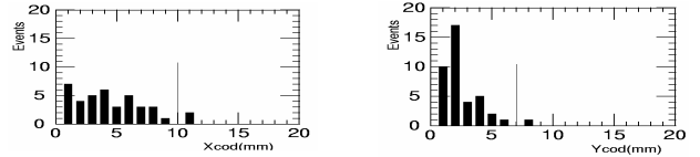
Figure 4 (a) COD distribution in the dipole with the max. \beta_x .
