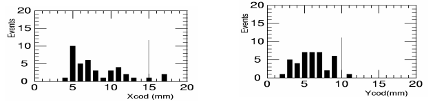
Figure 4 (b) COD distribution in the quadruple with the max. \beta_x .
