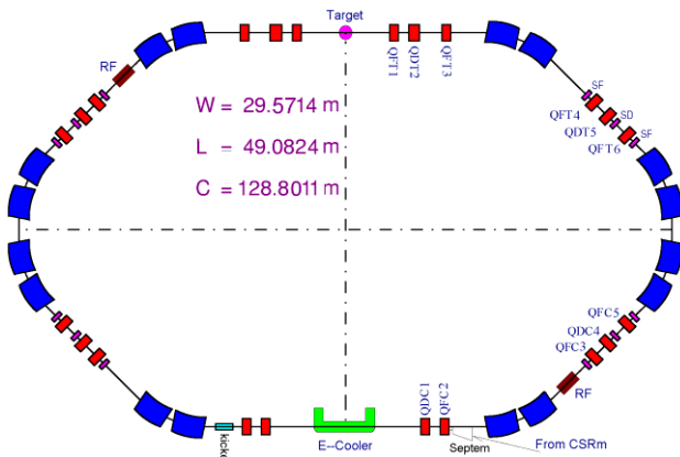
Figure 1: The layout of the CSRe
