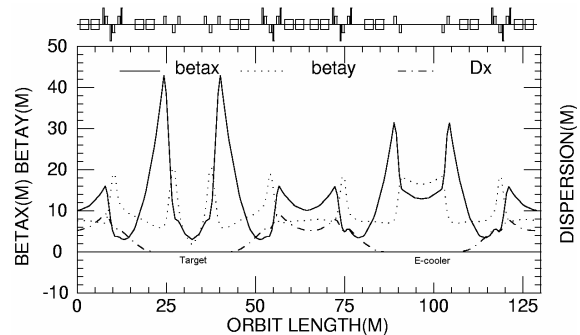
Figure 2 The distribution of the \beta -functions and the dispersion for the internal-target mode.
