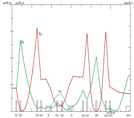
Figure 2. The beam optics of LBT
