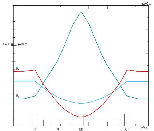
Figure 3. The beam optics of BS in a unit cell
