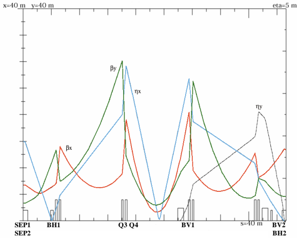
Figure 4. The beam optics of HBT
