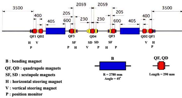
Figure 1. Layout of DBA-lattice (one unit cell) of storage ring
