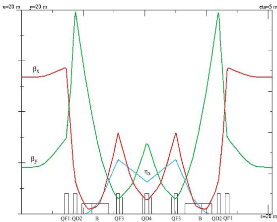
Figure 5. Beam optics of storage ring in a supercell
