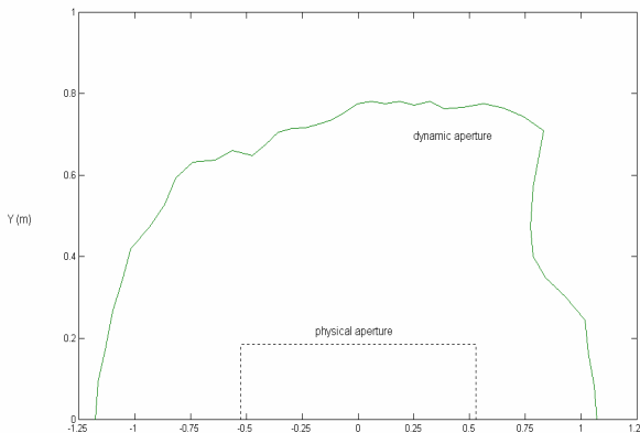
Figure 6. Dynamic aperture of storage in perfect status
