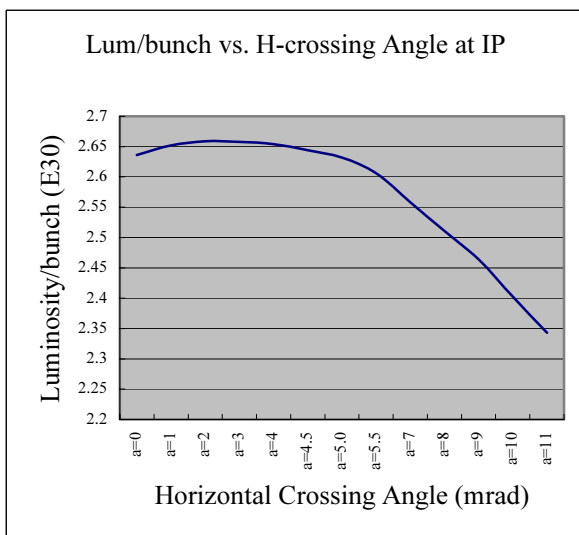
Figure 3: Simulation for parameters of April
