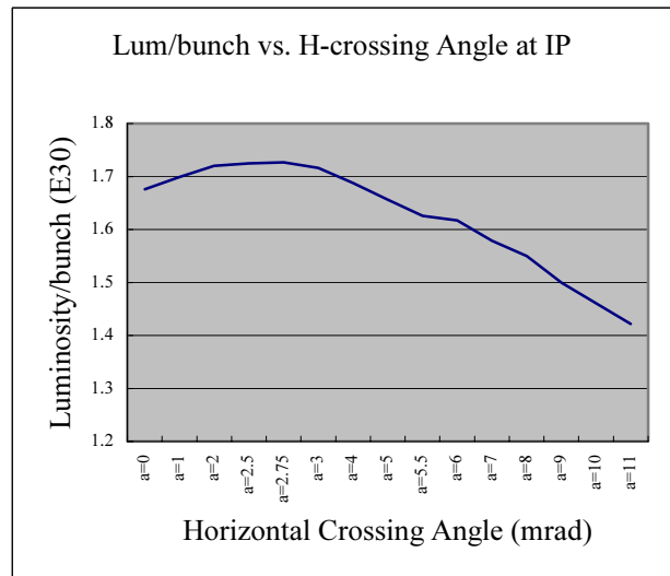
Figure 1: Simulation for the design parameters
