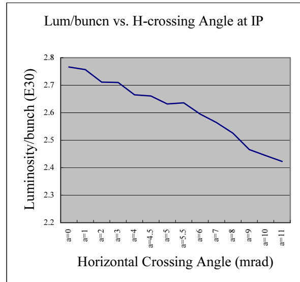
Figure 5: Simulation for parameters of February
