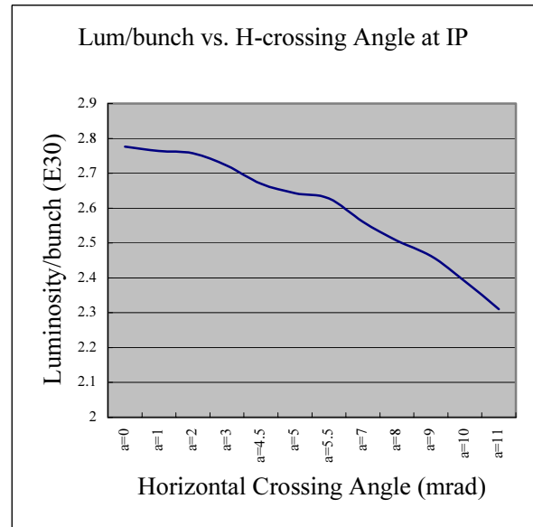
Figure 4: Simulation for parameters of May
