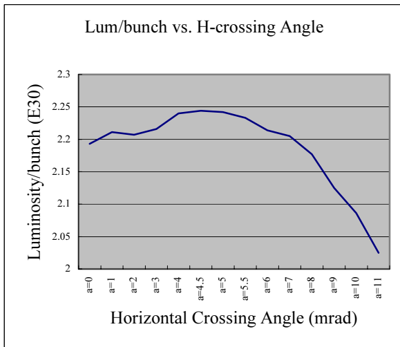
Figure 2: Simulation for parameters of March
