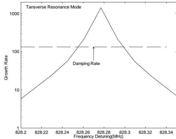
Figure 1: Growth rate due to the HOM with frequency 828.20 MHz
