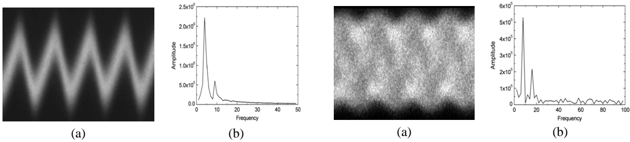
Figure 2: Sawtooth-like oscillation and FFT analysis result. In the streak camera image, the time scale of the horizontal axis is 1 ms and the vertical time scale means the bunch length. In the FFT analysis result, the horizontal axis is the frequency and the vertical axis is the amplitude. Frequencies of 4 kHz and 9 kHz are shown in the FFT analysis result.
