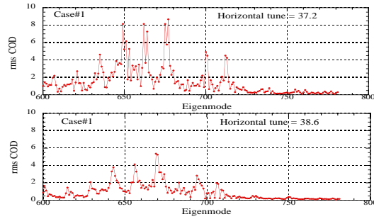
Figure 4: The COD response changes by the tune variation.
