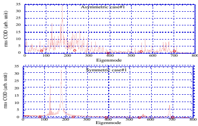
Figure 3-1: The rms COD for the 0.1 mm rms radial eigenmode offset of quads for the asymmetric (top) and symmetric (bottom) case#1.
