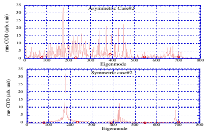
Figure 3-2: The rms COD for the 0.1 mm rms radial eigenmode offset of quads for the asymmetric (top) and symmetric (bottom) case#2.
