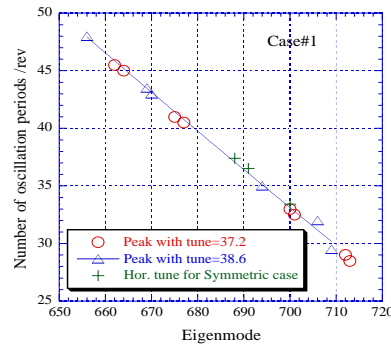
Figure 5: Peaks of the COD response shift to the different eigenmodes by changing the tune. Two symbols (circles and triangles) correspond to eigenmodes giving the peak COD response to two kinds of hor. tunes. For reference, tunes are shown with crosses for the symmetric case#1.
