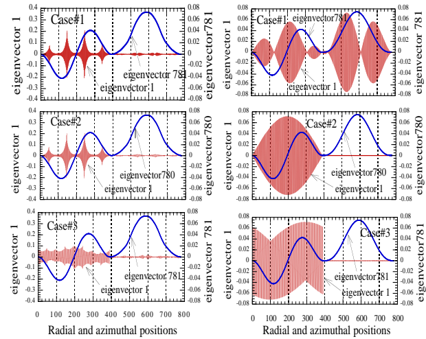
Figure 2: Eigenvectors with the largest (numbered as 1) and smallest (numbered as 781 or 780) eigenvalues for the asymmetric (left) and symmetric (right) cases. The left and right half of the eigenvector in each figure correspond to the radial and azimuthal displacements, respectively, to the order of quad arrangements. Case#1: upper, Case#2: middle, and Case#3: lower.
