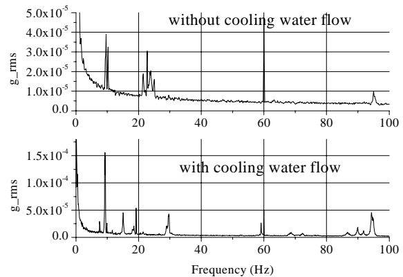
Figure 2 Frequency spectra of horizontal motions of the plate for manipulator with and without cooling water flow
