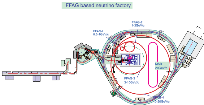
Figure 4: FFAG-based neutrino factory at the Tokai campus
