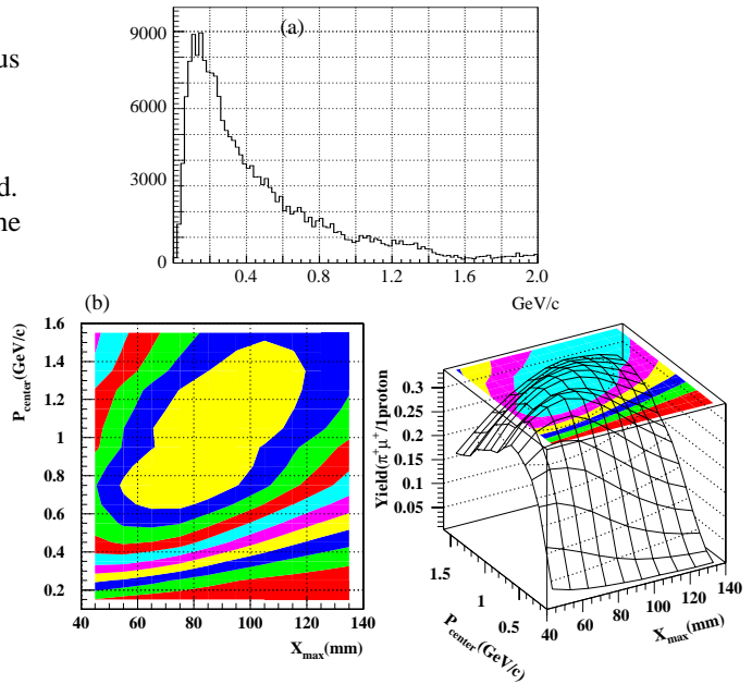
Figure 3: (a) Muon and pion distribution with fixed transverse acceptance( 10000\pi\text{mm}\cdot\text{mrad} ), (a)Total Momentum distribution (b) particle yield in various central momentum and beam size with fixed horizontal( 10000\pi\text{mm}\cdot\text{mrad} ) and momentum acceptance( dp/p=50\% )
