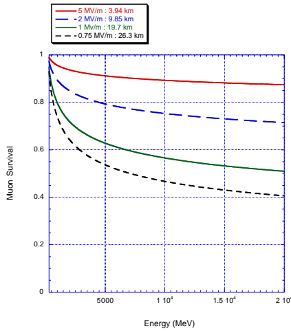
Figure 1: Muon survival rate during acceleration in various accelerating field gradient
