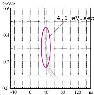
Figure 2: The particle distribution of the initial pion and the product muons generated by a short bunched 5 GeV proton beam in the longitudinal phase space. (Horizontal axis: time of flight(ns) Vertical axis:total momentum(GeV/c) )
