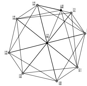
Fig.8 The survey network at the storage ring hall
