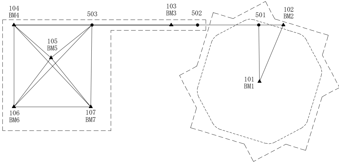
Fig.5 The Survey network for 1st order reference marks
