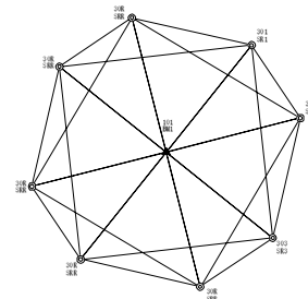
Fig.9 The computation of net adjustment for the alignment of storage ring
