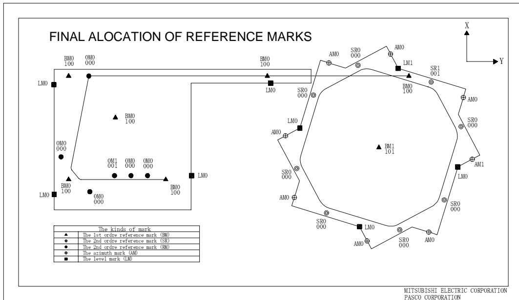
Fig.4 The allocation of monuments
