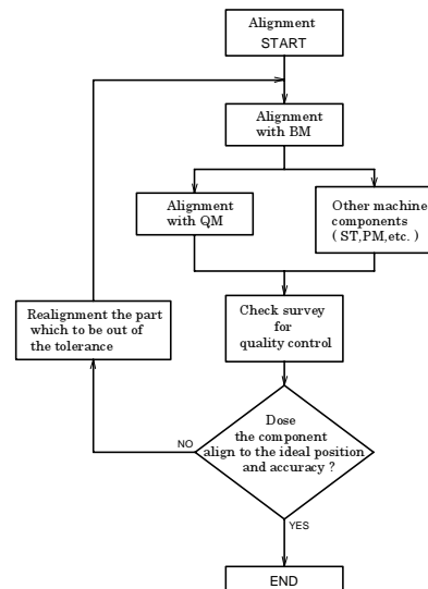
Fig.12 The flowchart of the alignment for the each storage ring component
