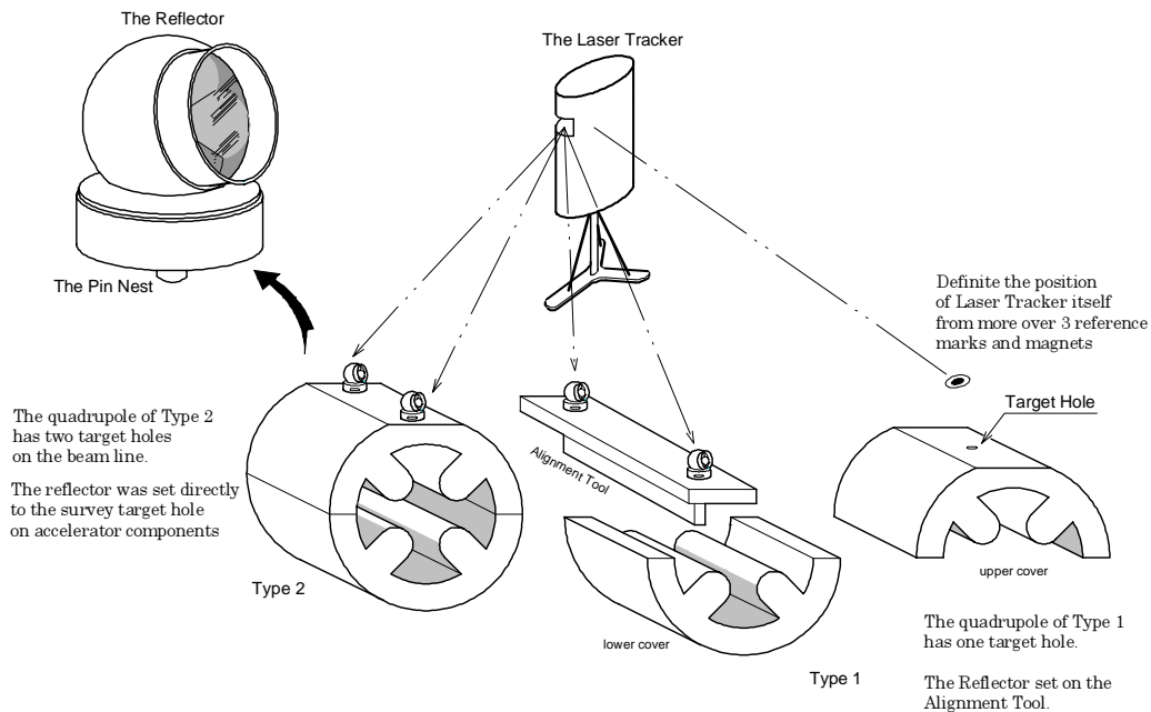
Fig.15 Scheme of alignment by the laser tracker
