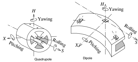
Fig.11 parameters for alignment
