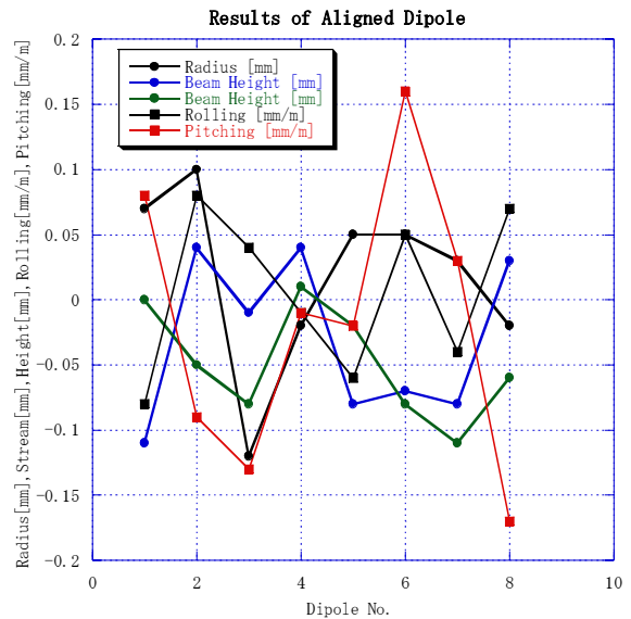
Fig.14 Results of the alignment for dipoles
