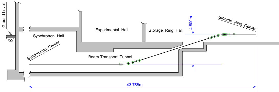
Fig.2 Profile of the accelerator complex of the SPS
