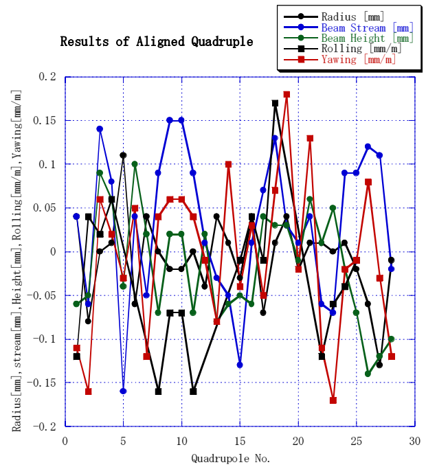
Fig.17 Results of the alignment for quadrupoles
