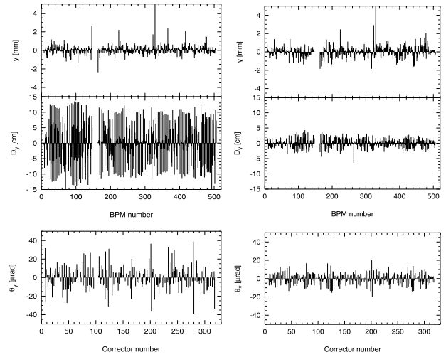
Figure 7: Measured vertical single beam orbit, dispersion, and corrector settings versus BPM number after standard MICADO steering (left) and after dispersion-free steering (right).
