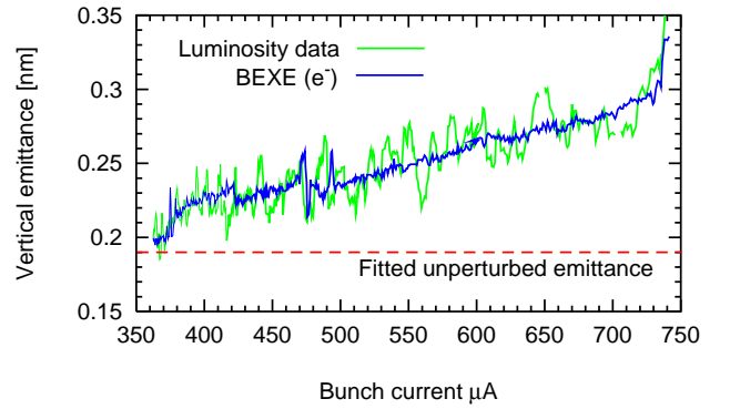
Figure 5: The vertical emittance as fitted and calculated from luminosity and synchrotron beam size measurements (BEXE) [24,25].
