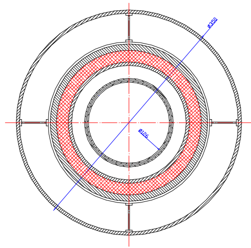
Fig. 4 The cross section of the magnet at SCQ
