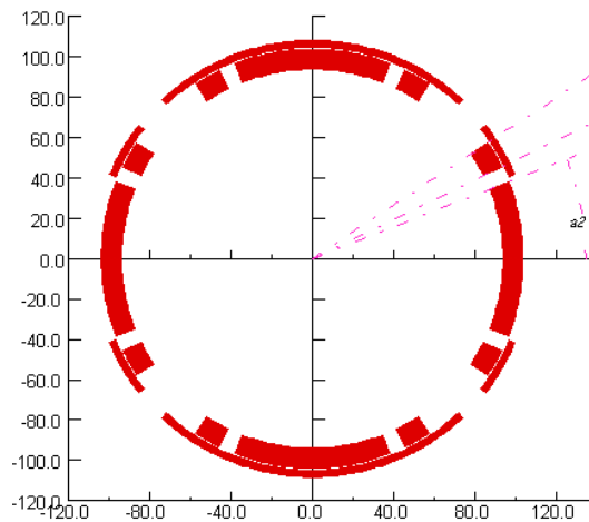
Fig. 2 Cross section of SCQ
