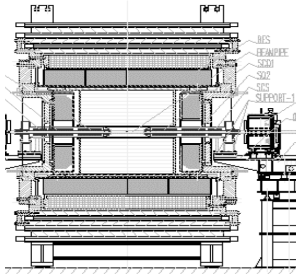
Fig. 8 Installation of BEPC-II IR Magnets
