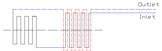
Fig. 6 circulation of cooling liquid helium in the magnet Quench Protection:
