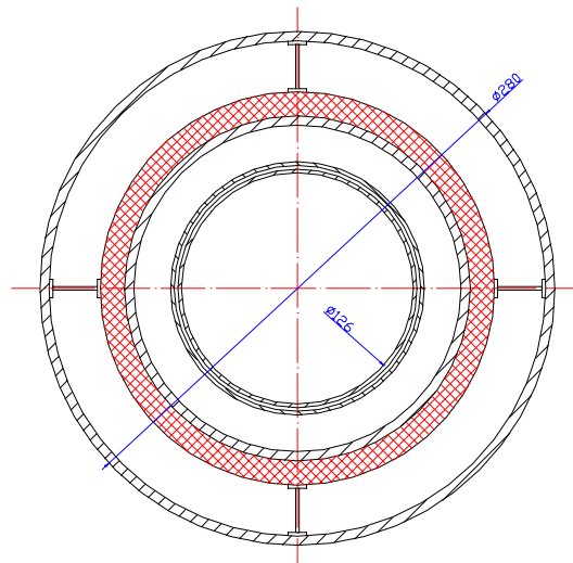
Fig. 5 The cross section of the magnet at SCB
