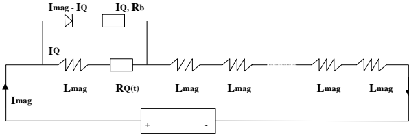
Fig. 7 Electric circuit of a quenching magnet in a magnet ring
