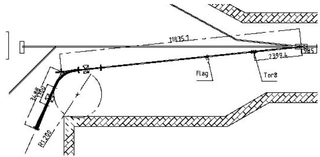
Figure 4: Final Redesign Layout
