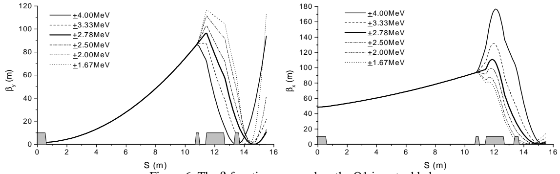
Figure 6: The \beta function curve when the Q1 is not added
