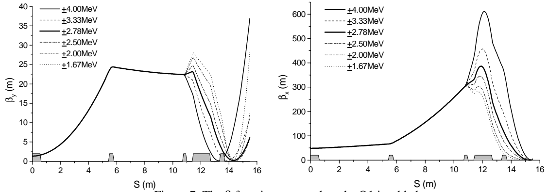
Figure 7: The \beta function curve when the Q1 is added
