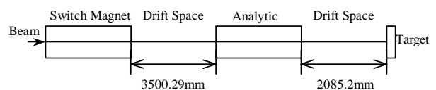
Figure 2: Lattice Sketch Map
