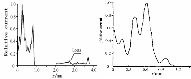
Fig.4. Beam distribution at the electron gun exit at the focusing electrode (Left: \phi_1=16.8\text{mm} , Right: \phi_1=13.8\text{mm} )
