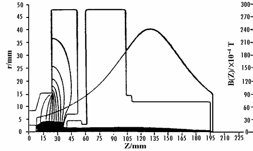
Fig.3. Electron trajectories in the electron gun at the focusing electrode ( \phi_1=16.8\text{mm} )
