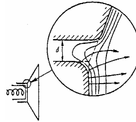
Fig.2. Disturbance of the edge electron trajectories, caused by the change of the distance between the cathode and the focusing electrode
