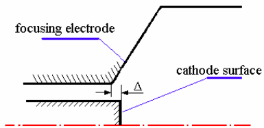
Fig.5. Relative position of focusing electrode and cathode
