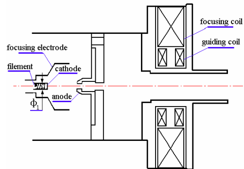
Fig.1. Electron gun structure
