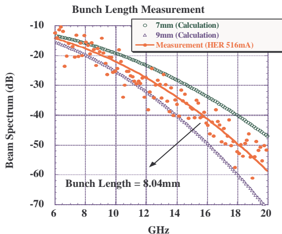
Figure 7: Frequency component picked up every 127MHz. And expected spectrum of several bunches length of the beam.
