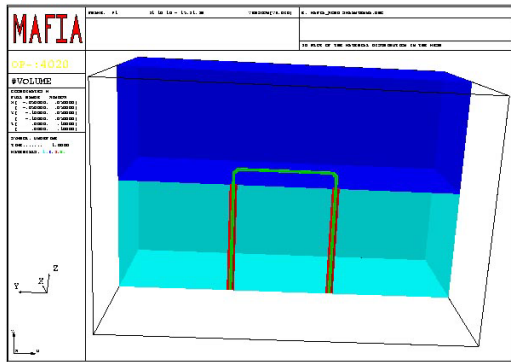
Figure 4: The Structure of the pick-up antenna. (The upper part of the box is inside of the waveguide.)
