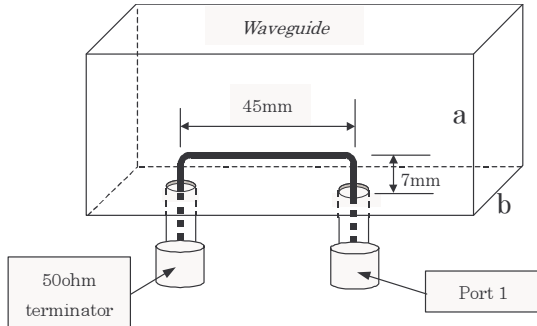
Figure 3: Sketch of the pick-up structure.
