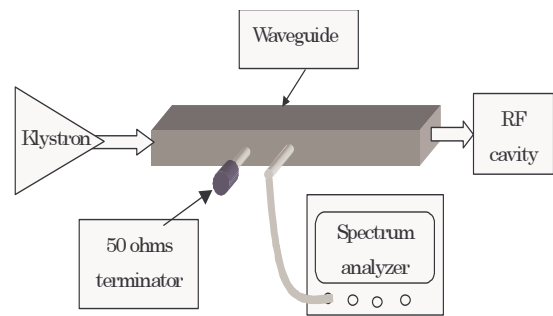
Figure 2: Sketch of the pick-up system
