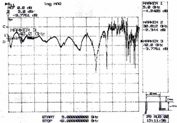
Figure 6: The testing result of S11 in the frequency range from 5GHz to 40GHz.
