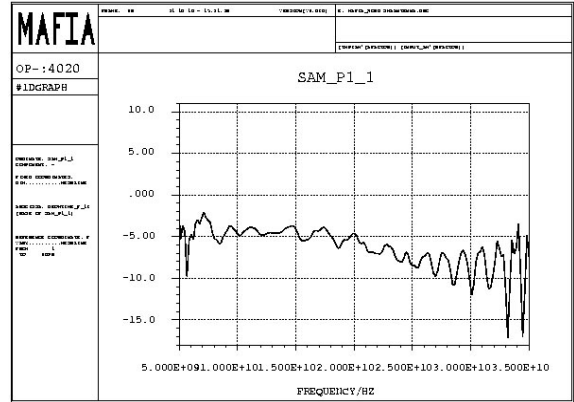
Figure 5: S11 at the input port of the pick-up in the frequency range from 5GHz to 35GHz.
