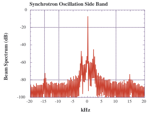
Figure 8: Synchrotron oscillation Side-band at KEKB LER
