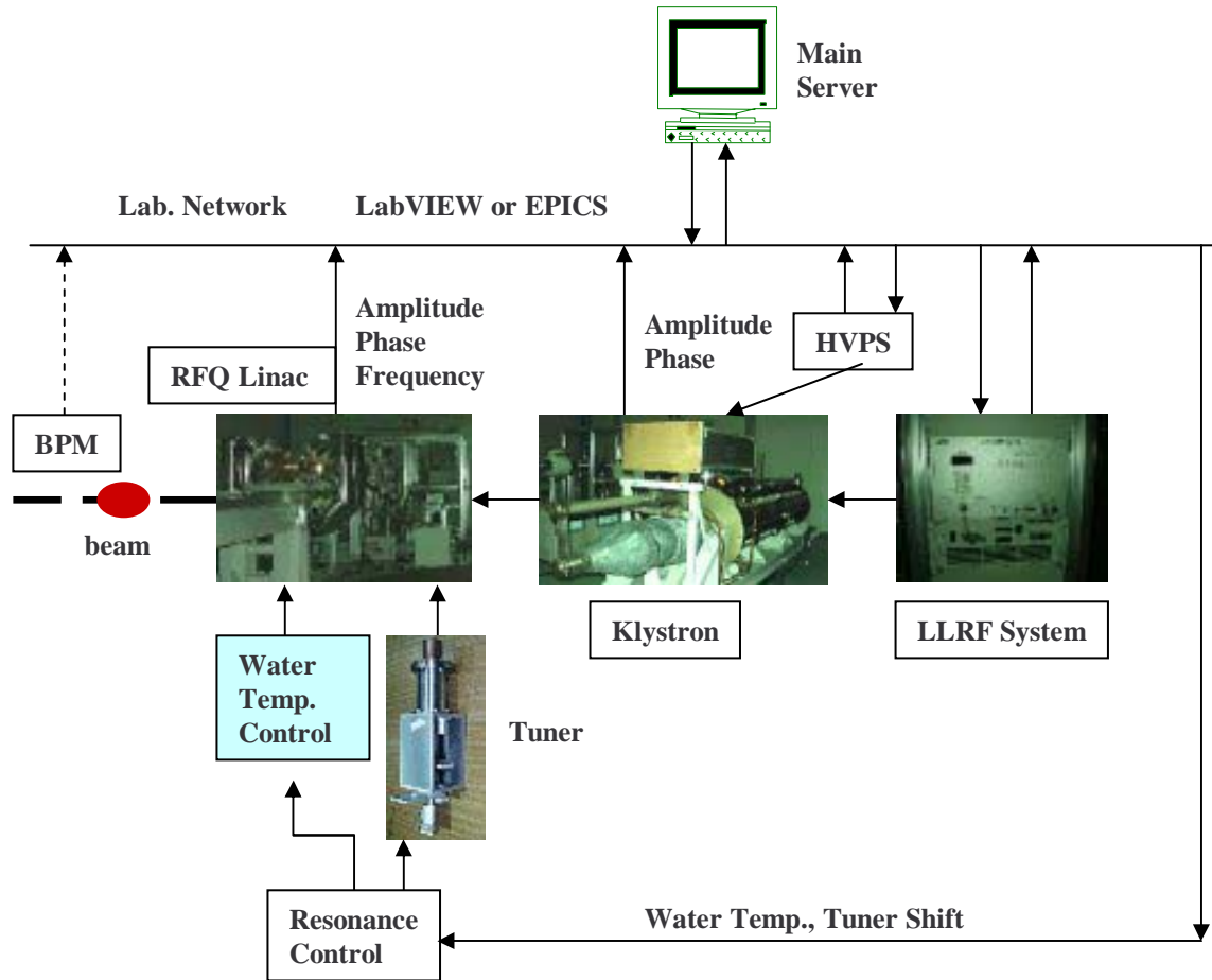
Figure 3. RF feedback loop.
