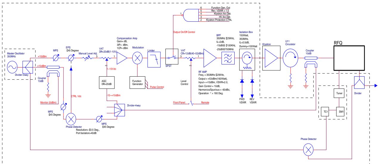
Figure 1. LLRF system for the KTF RFQ.
