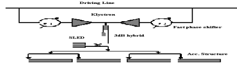
Fig. 4 RF system archeticture
