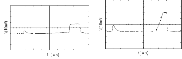
a) flat-top waveform b) RAMP waveform
