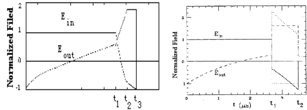
Fig. 2 Generate RAMP pulse Fig. 3 Generate Flat-top pulse
