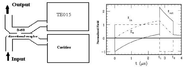
Fig. 1 SLED and its typical input and output waveform
