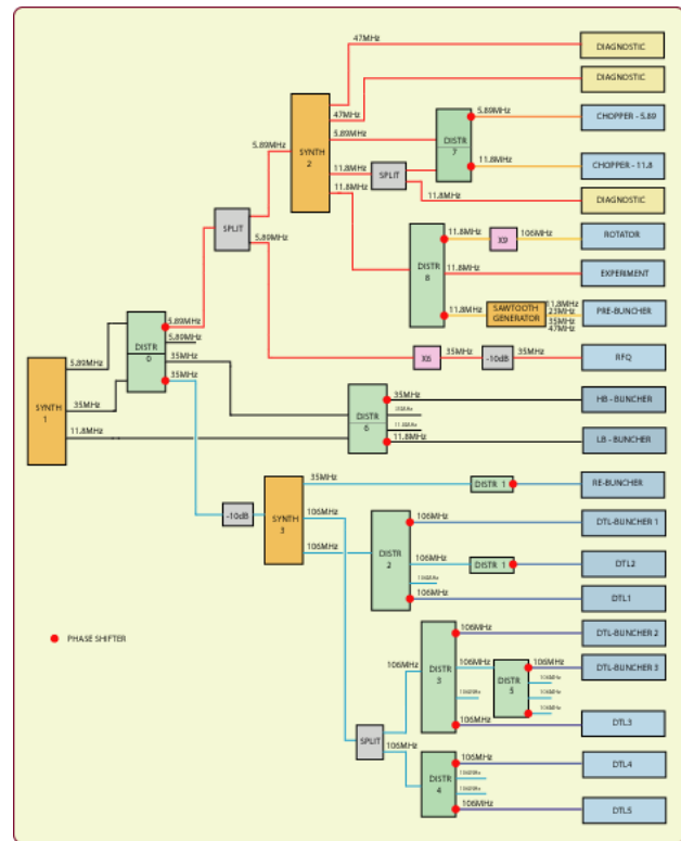
Figure 1-Block Diagram of Frequency Distribution System
