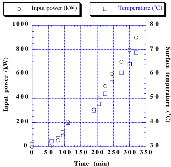
Figure 2: A typical result of the high power test for water-loads at KEK.
