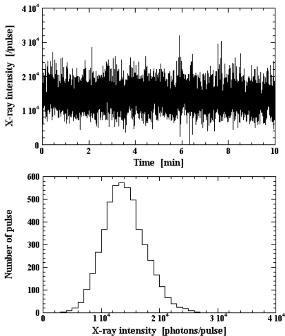
Fig. 4 The pulse-to-pulse fluctuation of the X-ray intensity.
