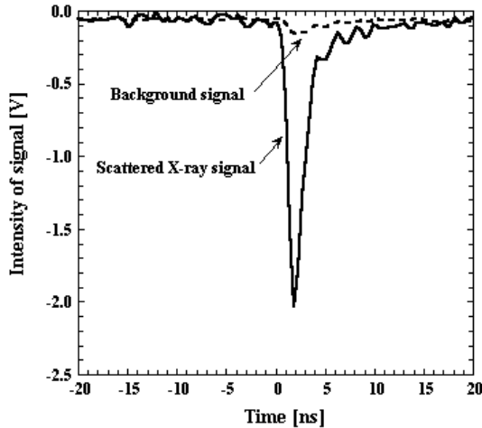
Fig. 2 The output of MCP signals
