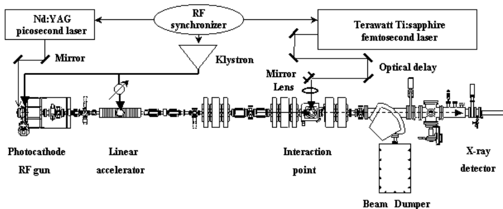
Fig. 1 A femtosecond X-ray source
