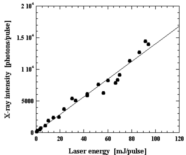
Fig. 3 The linearity of the X-ray intensity with the laser pulse energy.
