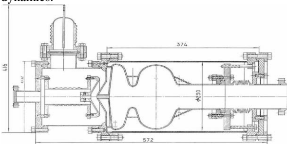
Fig. 2 Configuration of DC-SC photocathode injector
