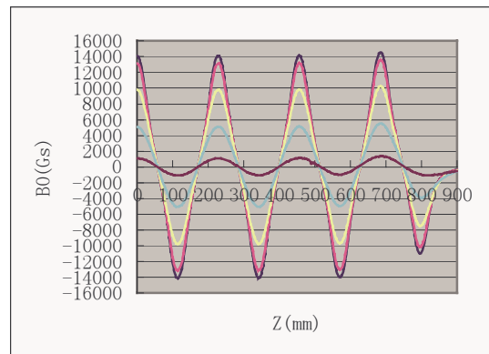
Figure 4: The magnetic field distributions at the midplane of 1W1
