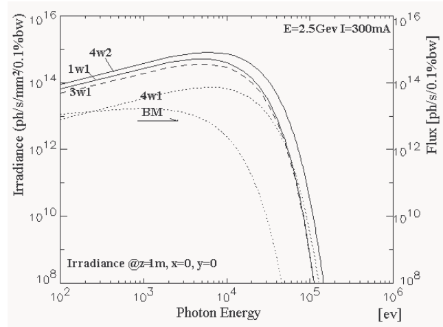
Figure 8: Irradiance calculated from wigglers at BEPC
