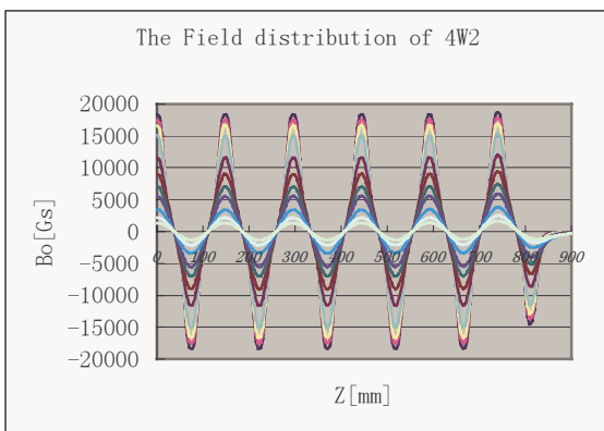
Figure 5: The magnetic field distributions at the midplane of 4W2
