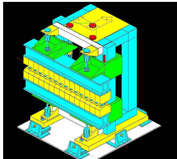
Figure 6: The 3D sketch map of 1W1
