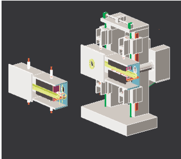
Figure 7: The 3D sketch map of in-vacuum wiggler(4W2)
