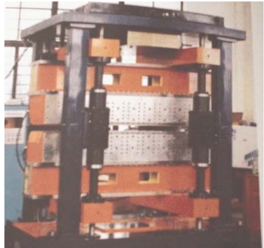
Figure 2: multipole permanent magnet wiggler 3W1
