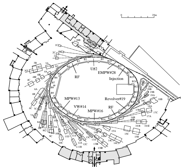
Figure 2: Layout of the Photon Factory storage ring.
