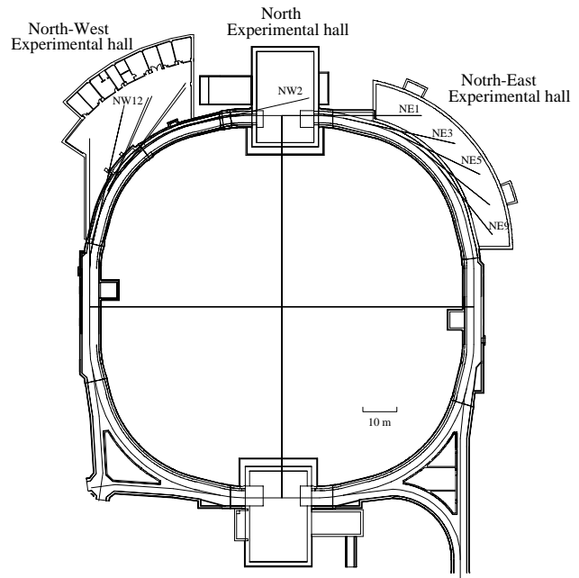
Figure 8: Ground plan of the PF-AR[26].
