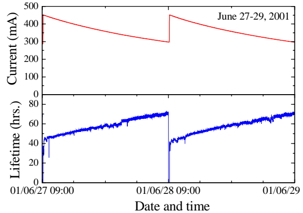
Figure 6: Beam current and beam lifetime during two days.
