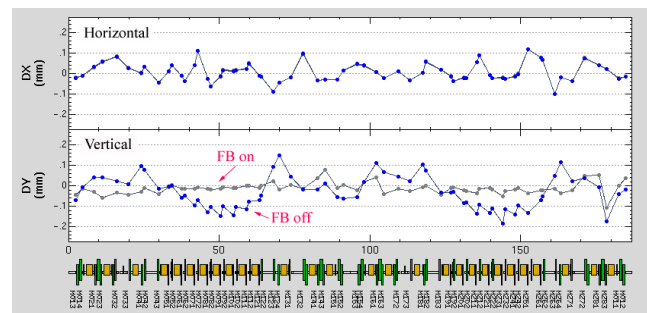
Figure 7: Beam positions with and without the feedback, which were taken 24 hours after the last COD correction.
