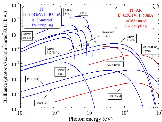
Figure 3: Brilliance of the synchrotron radiation[1].
