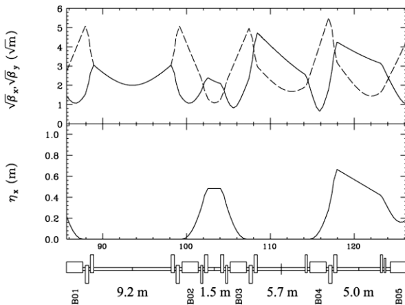
Figure 9: Beam optics in the straight sections after the upgrade.
