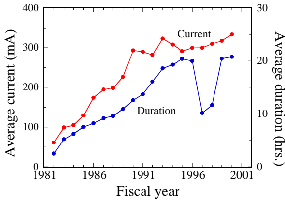
Figure 5: Average beam current (during multibunch user runs) and average duration of one user run.
