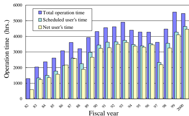
Figure 4: Summary of the operation time of the PF storage ring.
