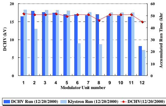
Fig. 2: Status of the PLS linac klystron-modulator.
