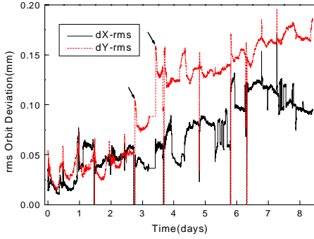
Fig. 5. RMS orbit deviation with operation time. Arrows indicate large increase of RMS values by the degaussing of magnets by unexpected beam dumps.
