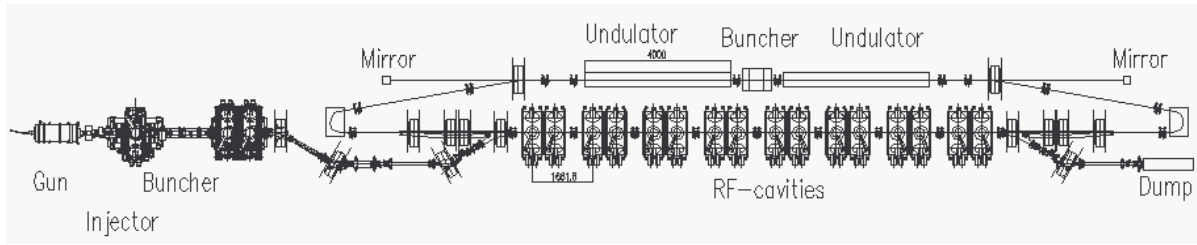
Figure 2: Scheme of the first stage of the high power free electron laser.
