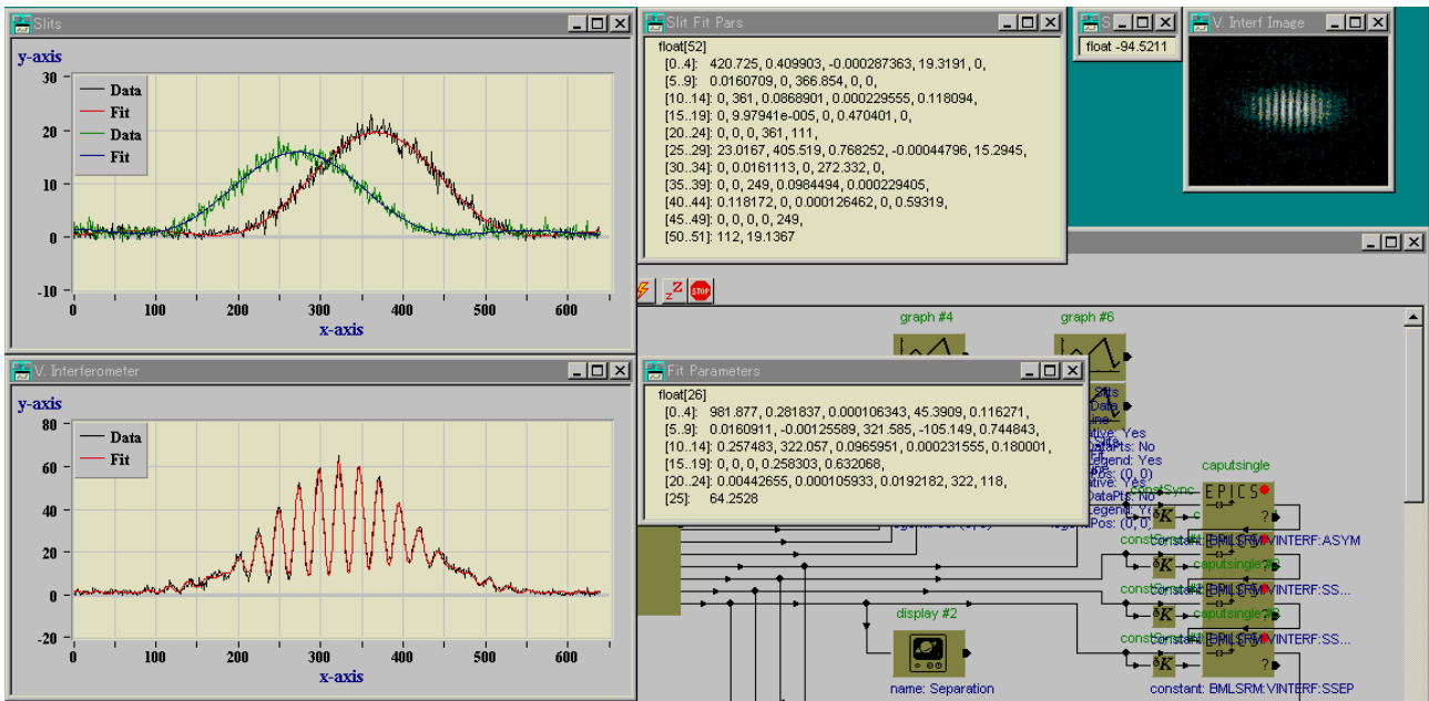
Figure 8: SR monitor data acquisition and analysis system. The curves in the upper left are the single-slit components of the interferogram measured with a shutter, and the lower curve is the resulting 2-slit interferogram. The separation and unequal heights of the single-slit peaks are the result of mirror distortions due to heating, and have to be corrected for to measure the beam size accurately.
