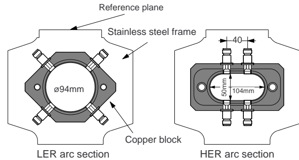
Figure 2: BPM block structure.
