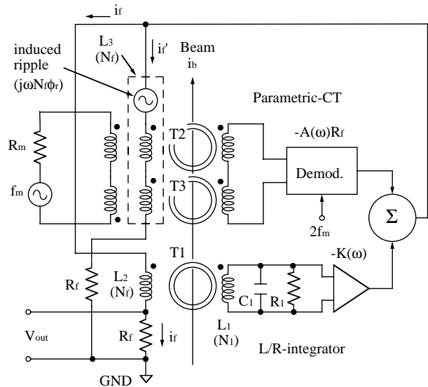
Figure 11: Block diagram of parallel-feedback DCCT.
