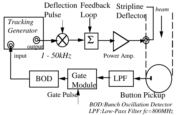
Figure 7: Block diagram of gated-tune meter.
