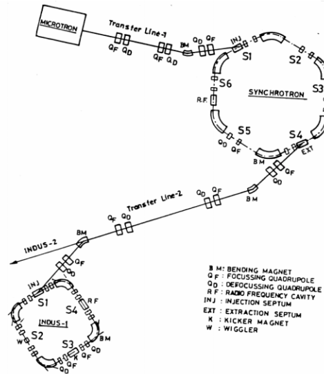
Figure.1: Layout of the Indus-1 SR facility
