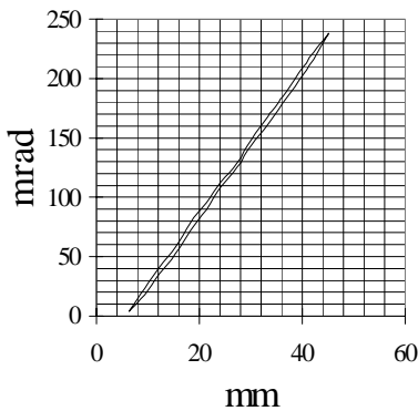
Fig3. Emittance plot of ion beam
