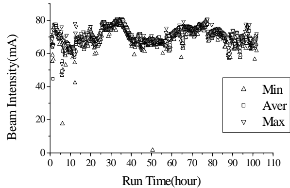
Fig4. Beam current Vs elapsed time 100 hours test
