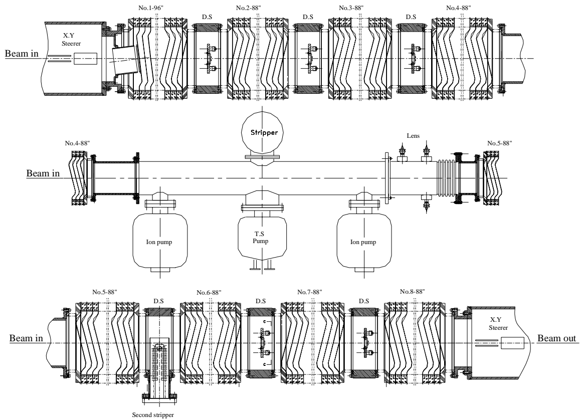
Fig.3 Tube up-Grading Configuration
