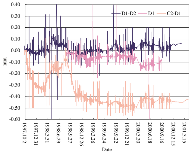
Figure 2. Motion of the borders of C2-D1, D1-D2 and D1 floor. Border of C2-D1 changed rapidly (in 50 hours) by about 0.15 mm in the middle of October 1997 and it increased gradually up to 0.35 mm for a few months. Many seismic vibrations (spike-like motion) were observed, but these are cut as complexity to see the graph after November 2000. Detailed explanation is written in the text.
