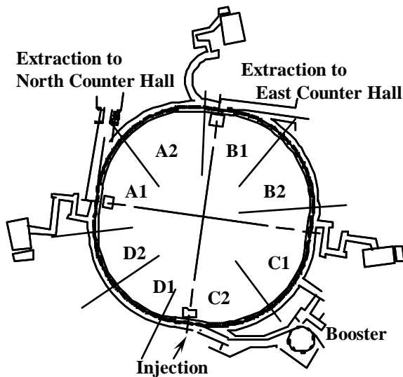
Figure 1. The main ring tunnel comprises eight separated floors.
