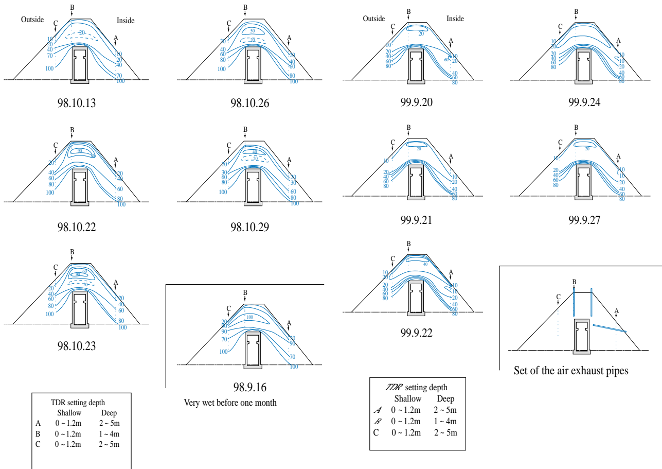
Figure 4: Contours of moisture in the soil bank in September 1999. It was rain of 27.5mm and 12.5mm for September 21 and 22. Just after rain, moisture of soil above the tunnel was only 40% and decreased to that of before rain after only five days.
