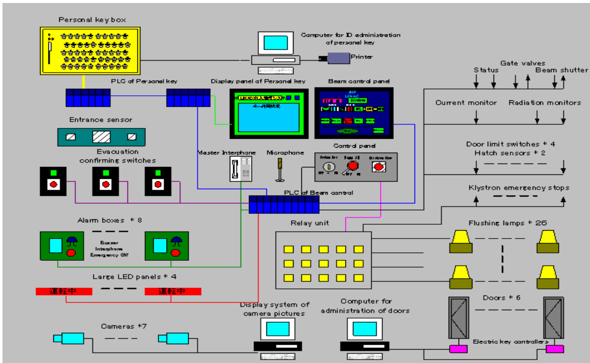
Fig.2 Control of the beam switch and construction of the safety system
