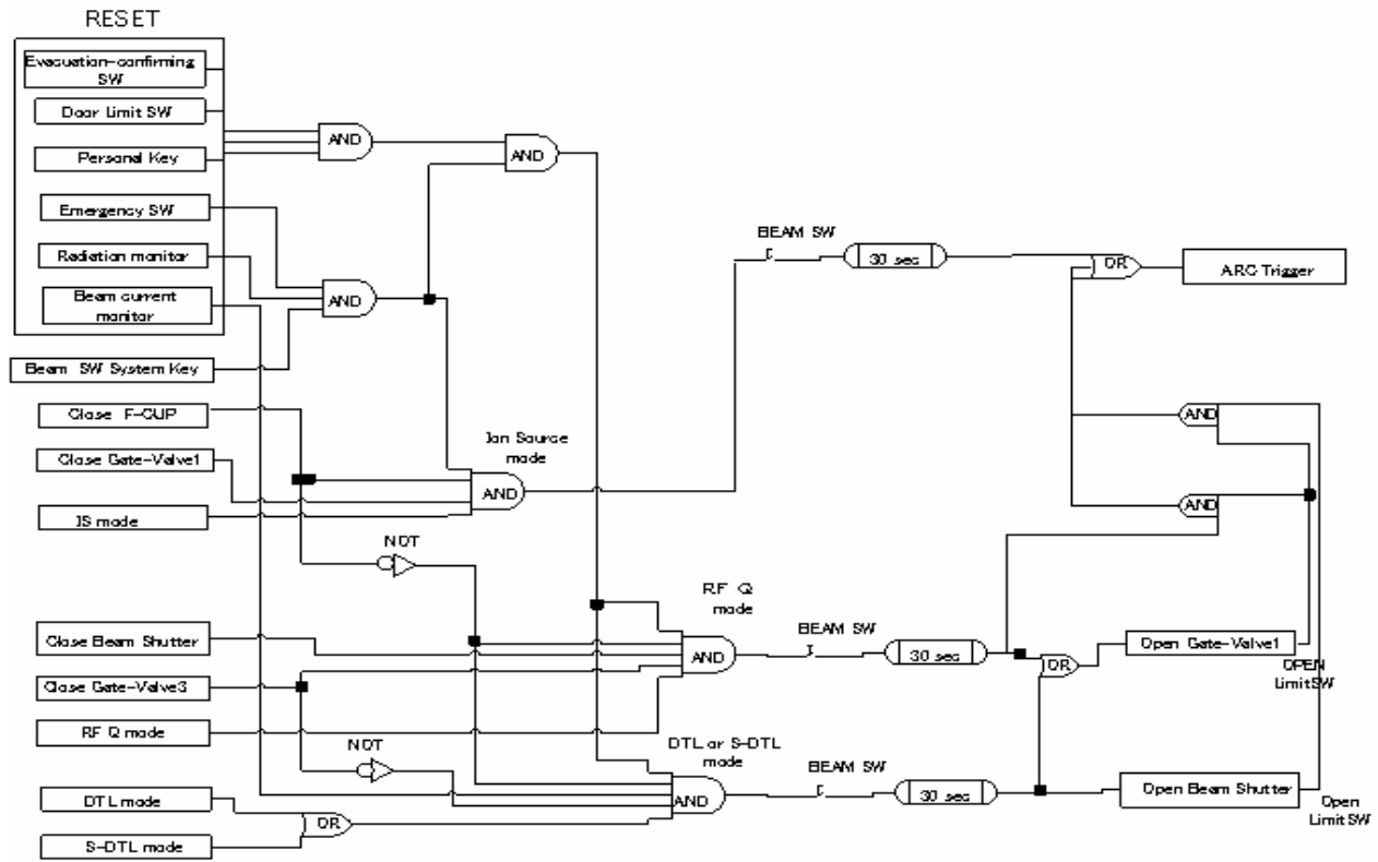
Fig.1 Upper figure: Beam Line Lower figure: The sequence of beam switch control
