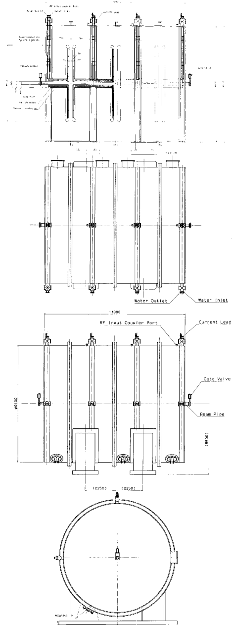
Fig. 5 Rough sketch of the \phi 9 \text{ m} cavity.
