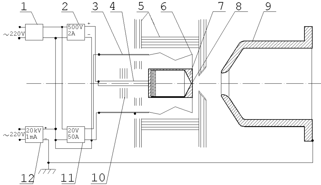
Figure 3: Ion source prototype schematic view. 1 - isolation transformer; 2 - direct current supply; 3 - cathode holder; 4 - container holder; 5 - thermal screens; 6 - cathode; 7 - container with graphite; 8 - emission hole; 9 - anode; 10 - additional thermal screen; 11 - cathode heater; 12 - accelerating voltage source.
