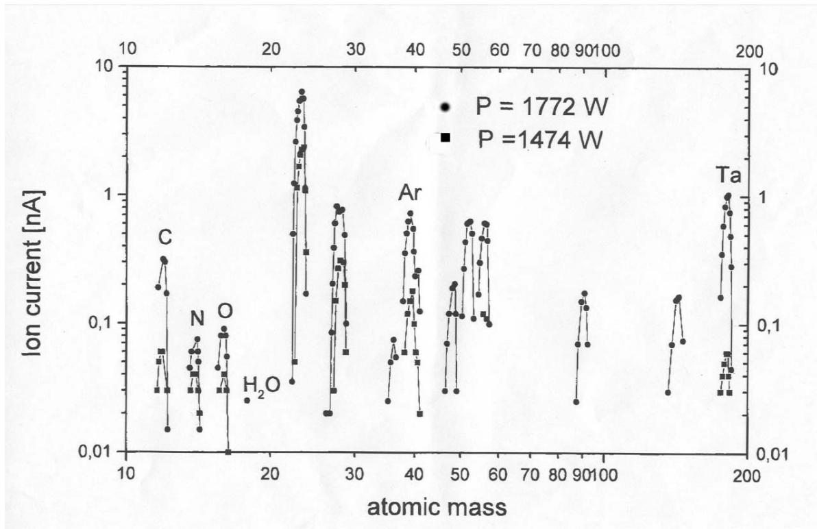
Figure 4: Ion current vs. atomic mass for various container's power supplies.
