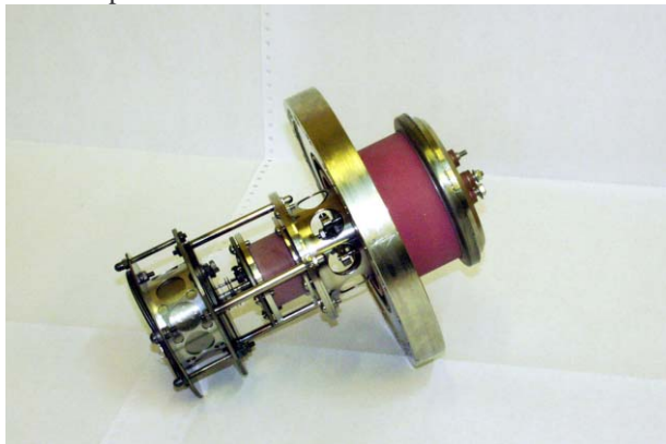
Figure 1: Picture of ion source prototype (side view)
