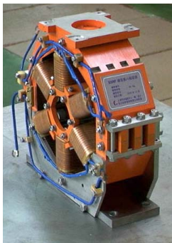
Figure 9: The booster sextupole prototype.
