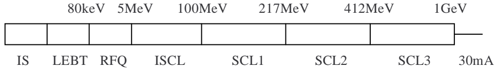
Figure 1: The block diagram of the ADS accelerator
