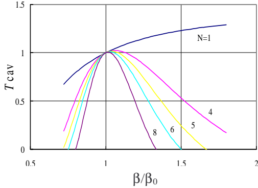
Figure2: The variations of T_{cav} with \beta and N .
