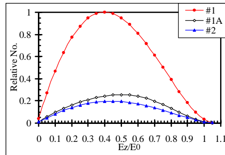
Fig. 8: Z-component energy distribution of the backstreaming electrons in klystrons #1, #1A and #2.
