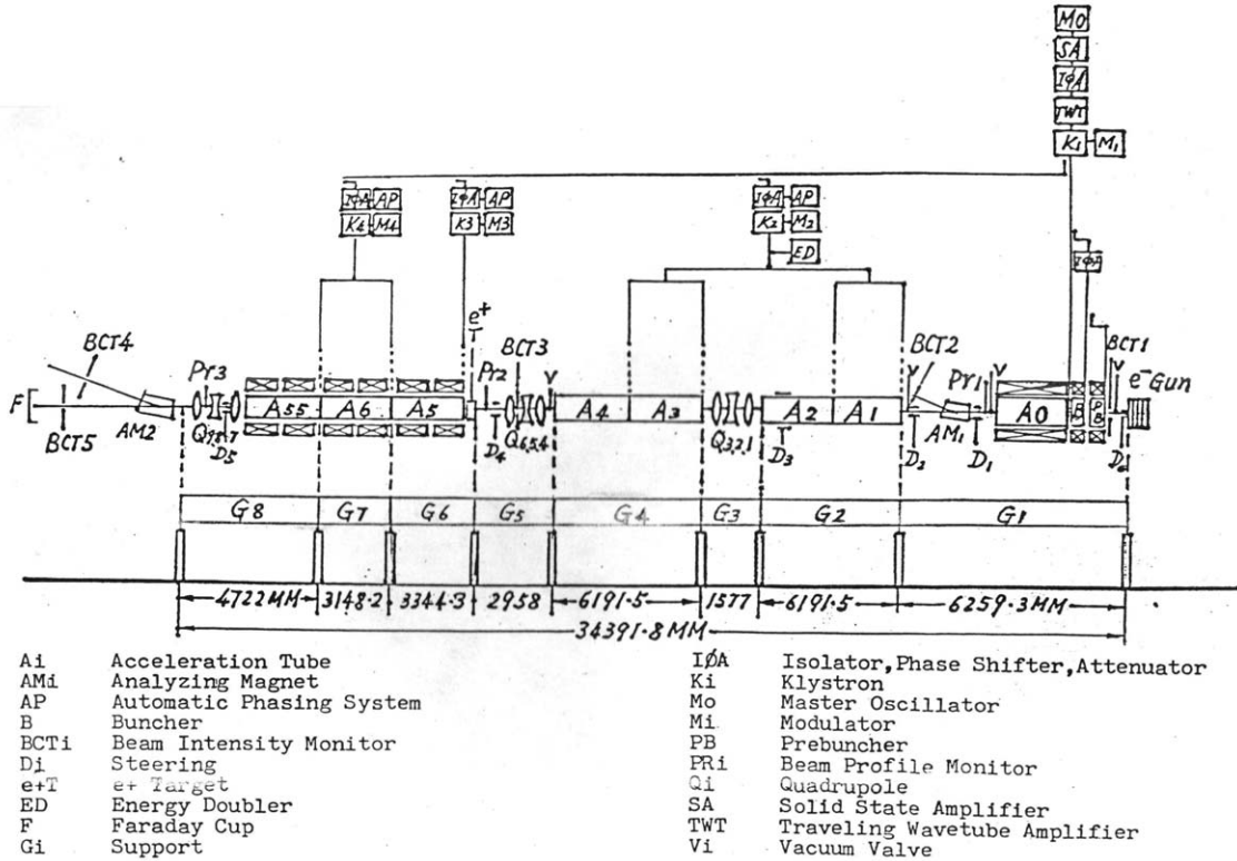
Figure 2 The schematic diagram of the BEPC 250MeV section.
