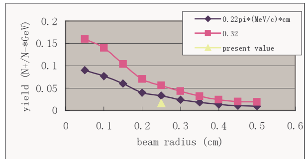
Figure 3 Positron yields as functions of electron beam radius
