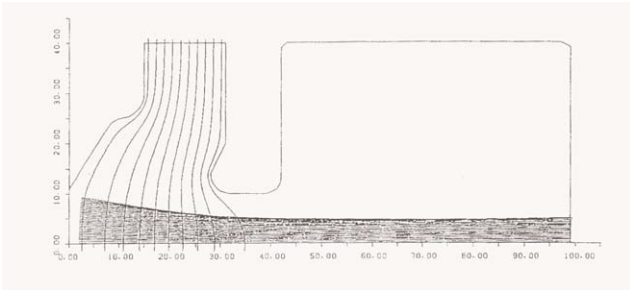
Figure 1 Computer plot of the gun optics at 160 kV showing equal-potential surfaces and the beam-focusing pattern. Shaded area denotes the electron beam. The emission current is assumed to be 12A.
