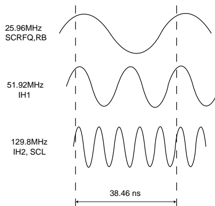
Figure 1 Time structure of beam bunch and rf fields.
