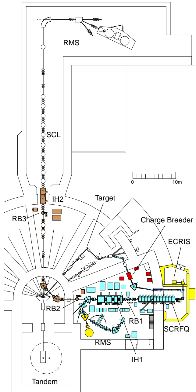
Figure 3 Layout of JAERI/KEK RIB Facility.
