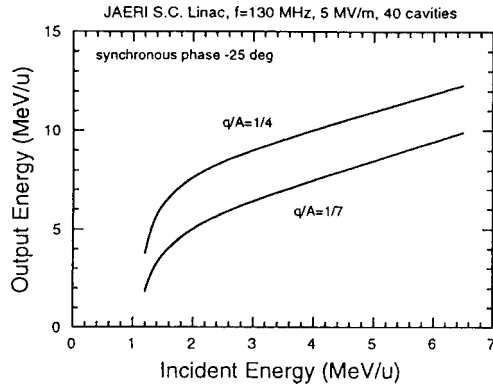
Figure 2 Maximum energy accelerated by the SCL as a function of incident energy.
