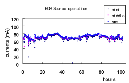
Fig. 3: 100 hours operation at 65mA/35kV
