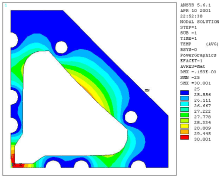
Fig. 5(a): Thermal and structure analysis for five cooling pipes
