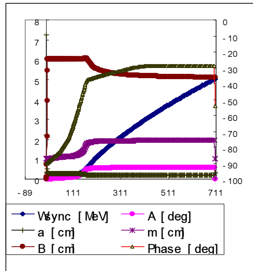
Fig. 4: main parameters of the RFQ
