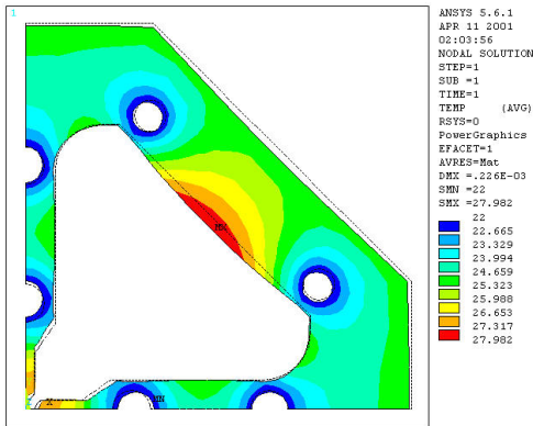
Fig. 5(b): Thermal and structure analysis for four cooling pipes
