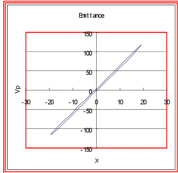
Fig.2: The measurement result of beam emittance ( W=30\text{keV} I=65\text{mA} \epsilon_{(\text{norm. rms})}=0.2\pi\text{mmmrad} )
