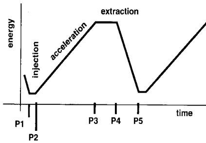
Figure 2: Typical machine cycle of 50-GeV main ring. P1-P2(injection):0.12s, P2-P3(acceleration):1.9s, P3-P4(extraction):0.7s, P4-P5:0.7s, total:3.42s. Slow extraction of 50-GeV, duty factor:0.20, average current:15.6 \mu A.
